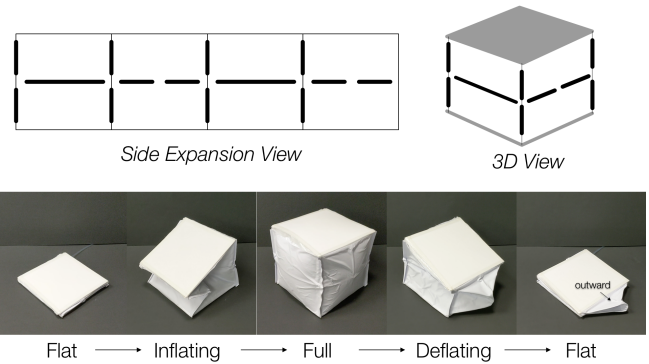
Figure 3. Box packaging folding. One possible folding outcome where the sides of the cube fold outward. (Thick lines in the illustration indicate acrylic tubes.)
